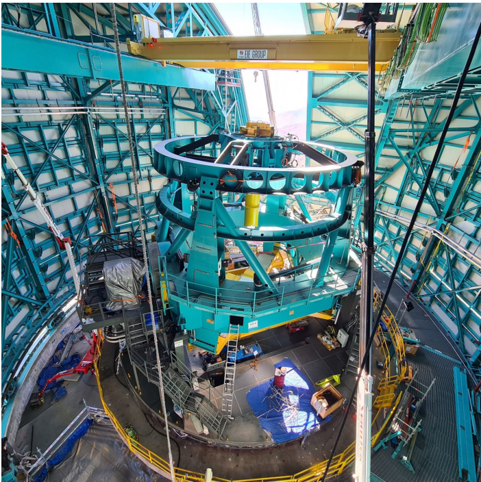
The interior structure of the Rubin Observatory's dome will hold the Simonyi Survey Telescope and the LSST Camera. (Rubin Observatory/NOIRLab/NSF/AURA)
